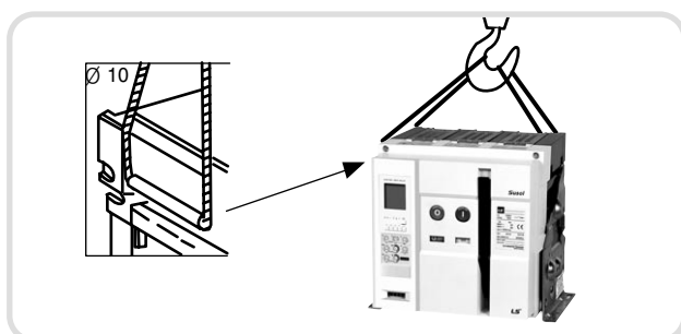
Fig. 2. Transporting method of Fixed type
