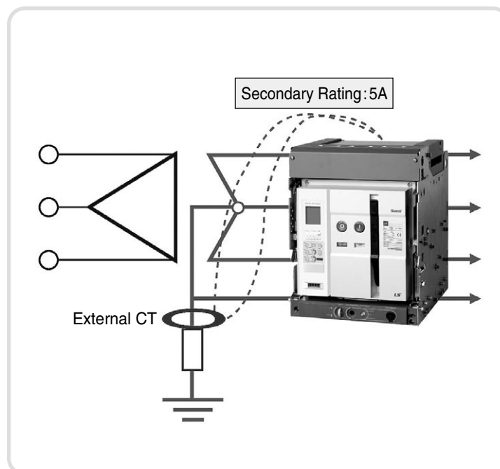
External CT Type Wiring 2
