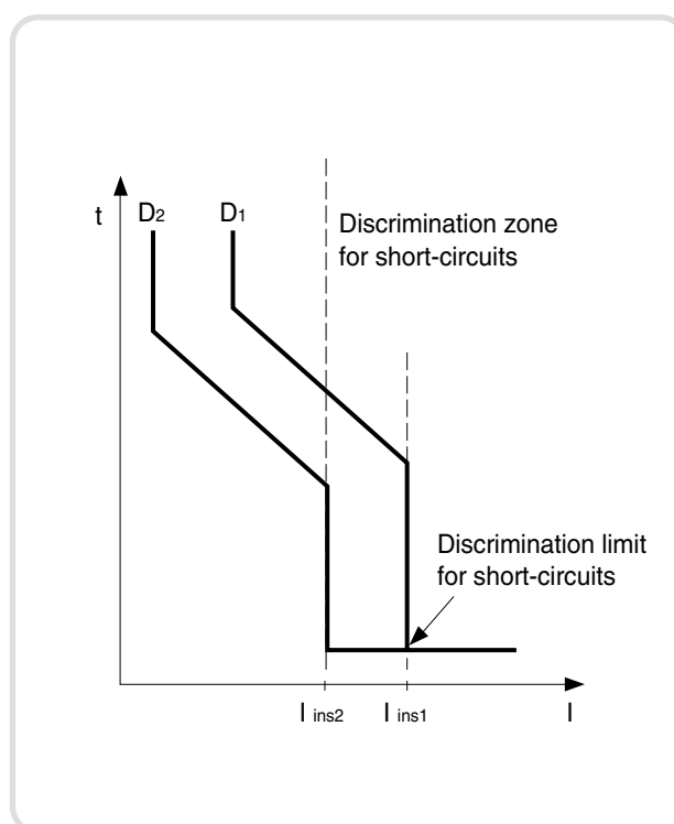
Picture 3. Current Selectivity
