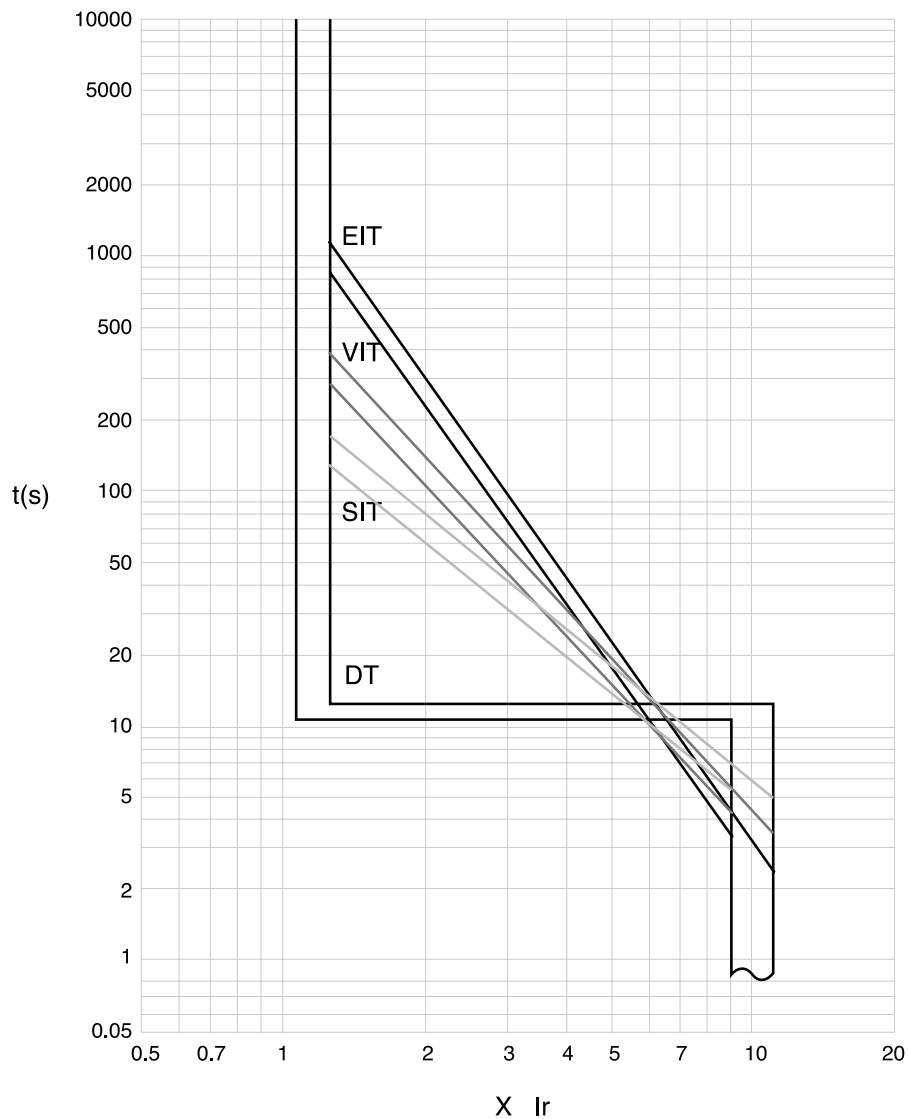
Picture 8. Characteristics of IDMTL
