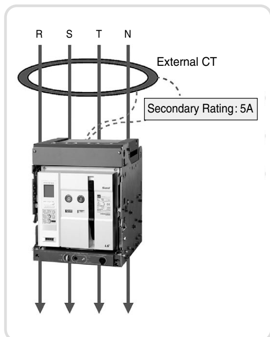
External CT Type Wiring 1
