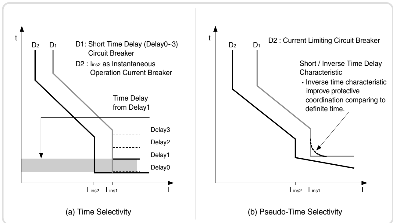
Picture 4. Time Selectivity
