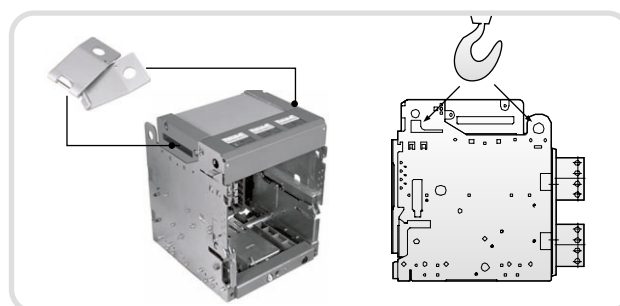
Fig. 3. Transporting method of Draw-out type
