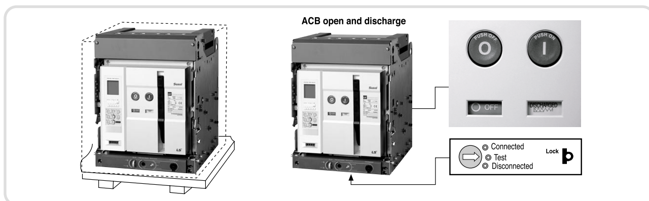
Fig. 4. Storage method
