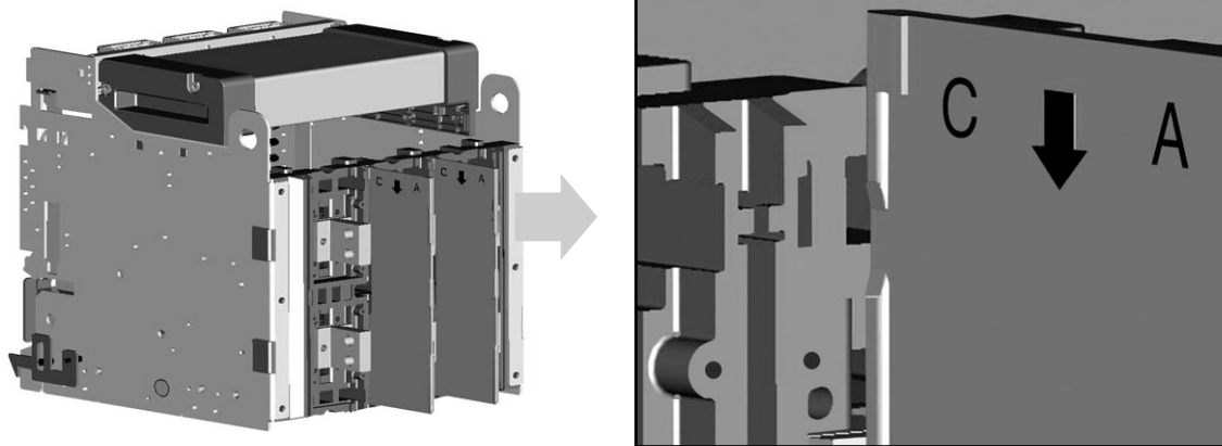
Draw-Out Type
