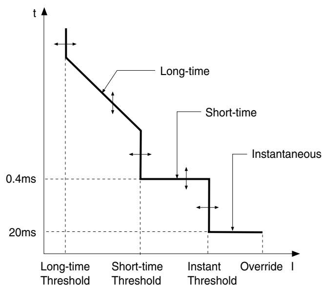
Picture1. Low Voltage Circuit Breaker's Characteristic Curve
