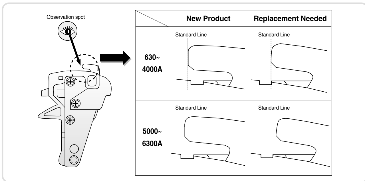
Fig 8. The standard figure for contact replacement
