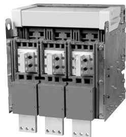
Fig.4 Vertical/Front type
