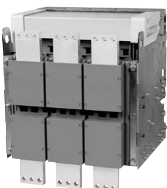
Fig.6 Front type
