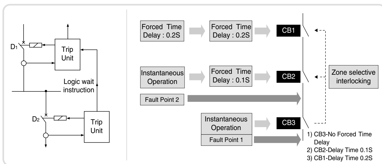
Picture 6. ZSI Operation Principle
