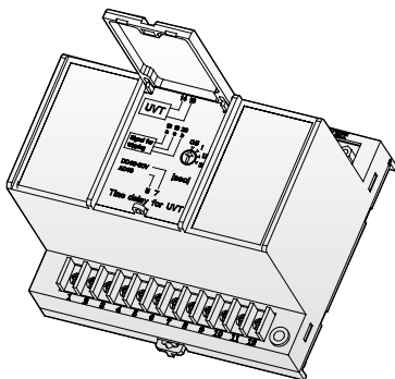
External Configuration
