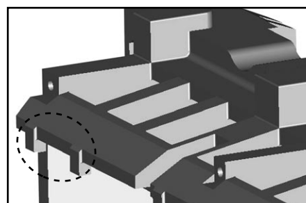
Projections for Assembling Shutter of BASE
